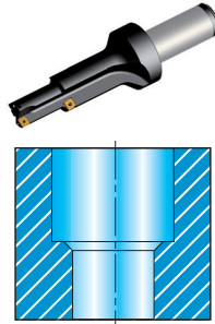
B5. Counterbore and chamfer
