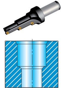
B6. Counterbore with chamfers
