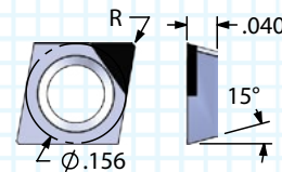
80° DIAMOND CBN/PCD TIPPED
