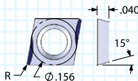
80° DIAMOND CHIP CONTROL RIGHT HAND ONLY
